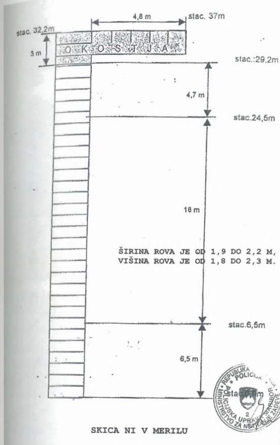
Skica rova B (RG-ING)
