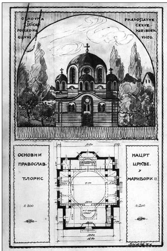
Skica in tloris pravoslavne cerkve v Mariboru (PAM SI_PAM/5, aš 292/27576)
